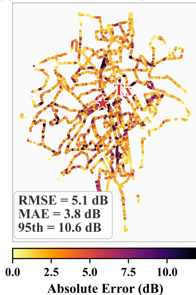
(c) Prediction Error (Test Set)
