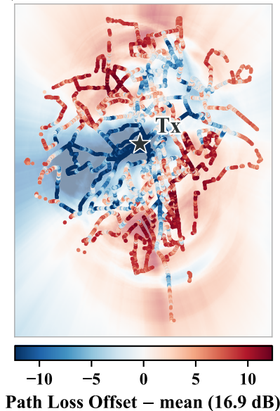
(b) Learned Path Loss Offsets
